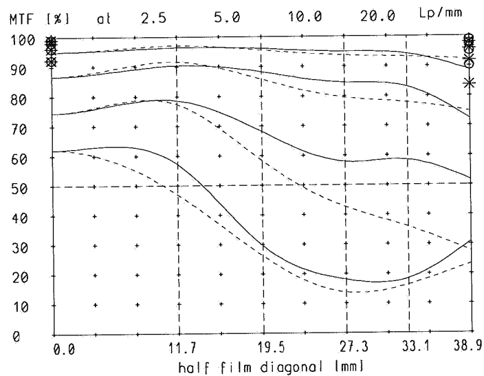
MTF at ratio 4x f/ 4.5
