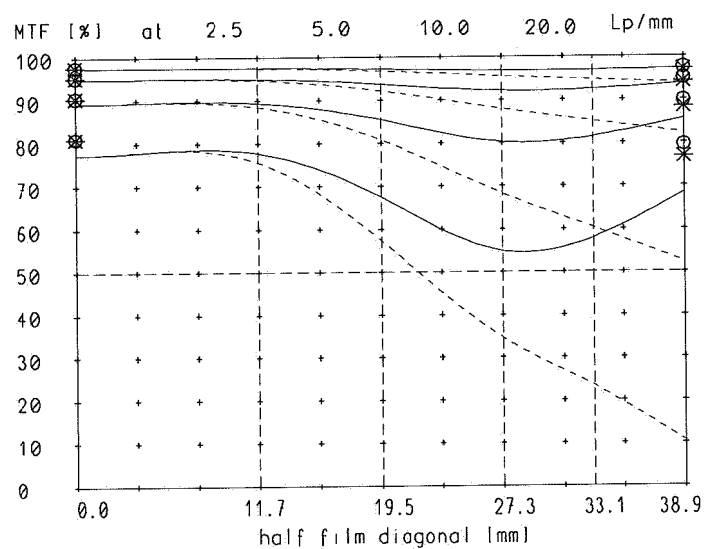
MTF at ratio 4x f/ 11
