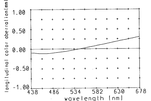
Longitudinal color aberration at ratio 4x
