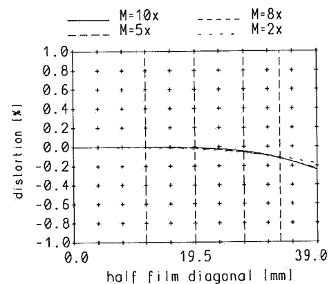
Distortion at ratio 10x to 2x
