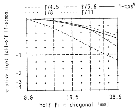
relative light fall-off at ratio 4x
